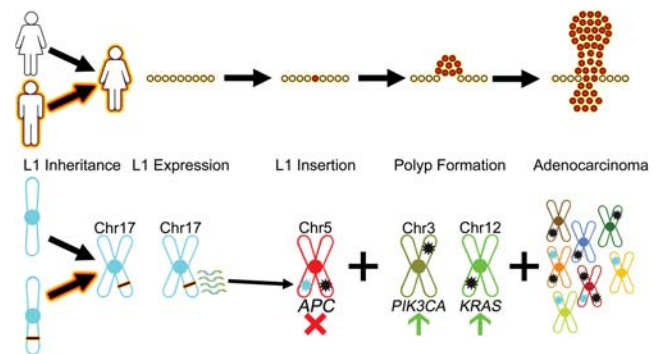
Figure 6. An oncogenic hot L1 evades somatic repression and initiates CRC. L1 Inheritance: Inheritance of a hot FL-L1s source element begins the process of L1-mediated cancer (this study). In this case, the patient inherited an African-specific hot FL-L1s source element on Chromosome 17 (black bar with fire outline, bottom) from one of her parents. L1 Expression: The inherited FL-L1s source element evades somatic repression and generates transcripts (squiggle lines, bottom) in normal colon tissues (this study). L1 Insertion: A somatic L1 offspring element is integrated into the sixteenth exon of the APC gene, thereby disrupting one APC allele (light blue star on Chr 5, bottom; this study) (Miki et al. 1992). The second APC allele is disrupted by the somatic mutation p.R1450* (black star on Chr 5, bottom; this study). Thus, both gatekeeper APC alleles are disrupted and the adenoma phase is initiated. Polyp Formation: Following loss of APC function, additional important driver mutations in the PIK3CA and KRAS genes (black stars on Chr 3 and Chr 12, respectively, bottom) result in progression to adenocarcinoma (cluster of red cells, top). Adenocarcinoma: Additional driver and passenger mutations occur to further drive progression of adenocarcinoma. These changes include new somatic L1 insertions (light blue stars, bottom), SNVs and indels (black stars, bottom), and perhaps other structural variants.
